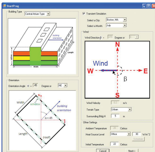
Pictured above is the user-interface for CoolVent, a simplified, early-stage building design tool for assessing natural ventilation. Source: MIT Building Technology Department.
