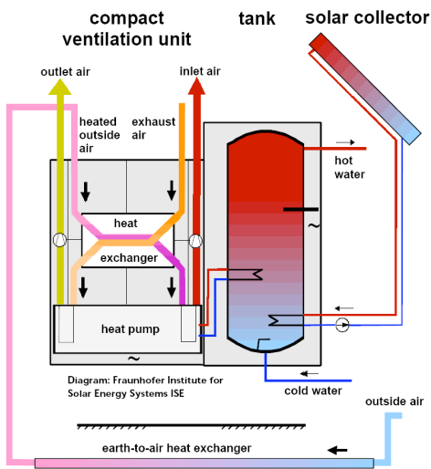
One of thousands erected in central Europe, the solar passive house (top) uses thick insulation and triple-glazed windows to keep annual heating loads below 15 kWh/m 2 . This building is equipped with a newly designed compact heating and ventilation device (left) that integrates solar thermal collection, earth heat exchanger, heat pump, and heat recovery systems to efficiently provide domestic hot water, space heating, and ventilation. Source: Fraunhofer ISE.
